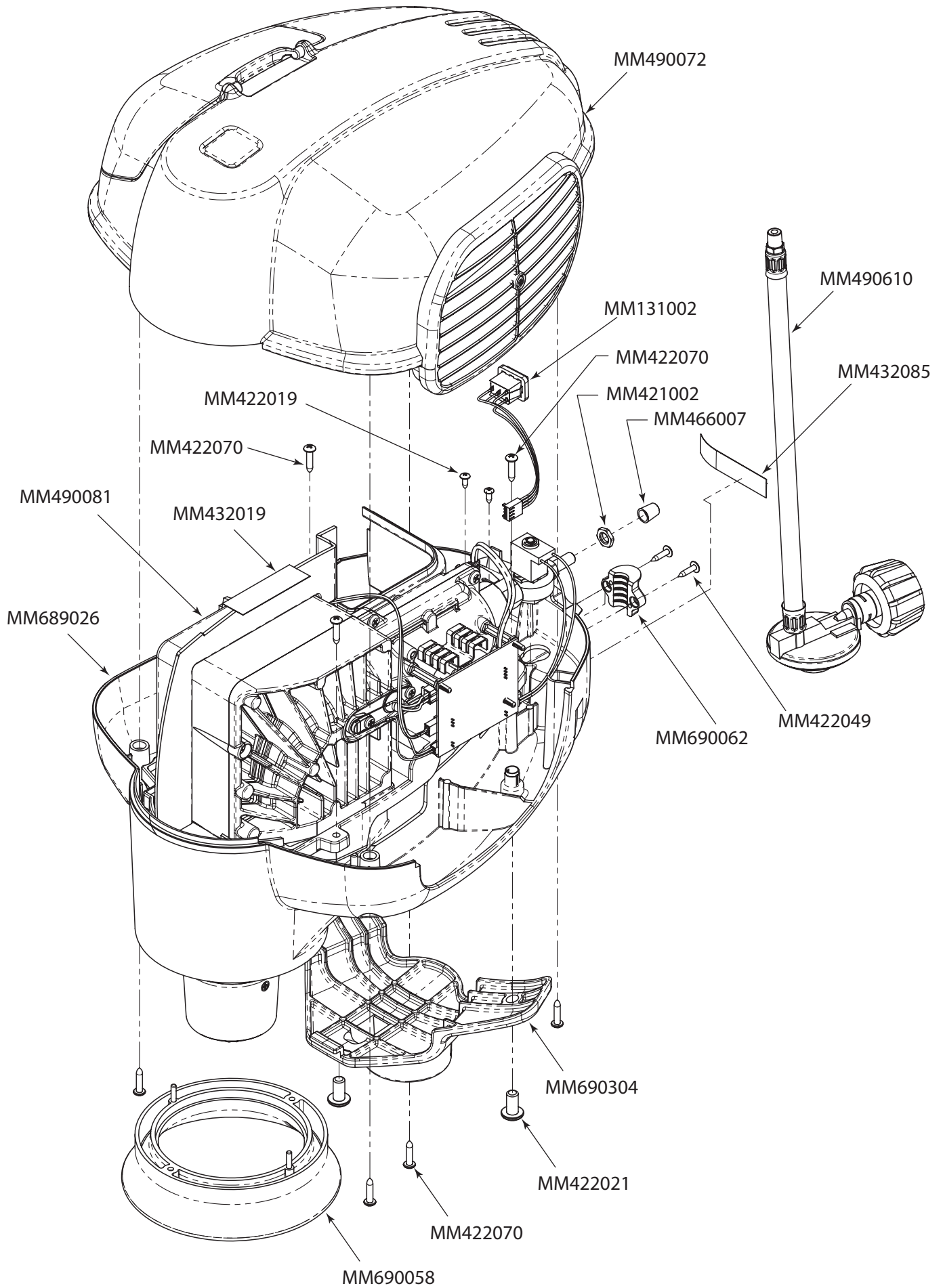
Housing Assy
